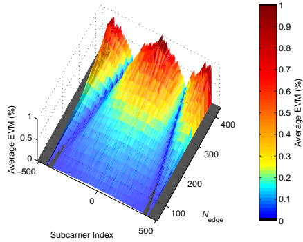
(e) Delay-spread based scheduling.
