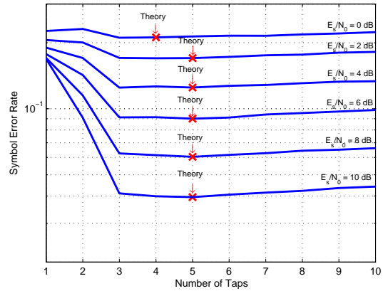
(b) Gaussian (NOFDM, \rho = 0.4 ).
