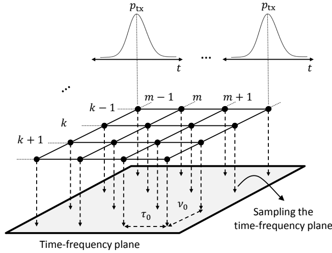
(b) Sampling the time-frequency plane. Modulated pulses are placed into the time-frequency plane, based on the locations of samples. In the illustration, the product of 1/\tau_0\nu_0 corresponds to the lattice density.
