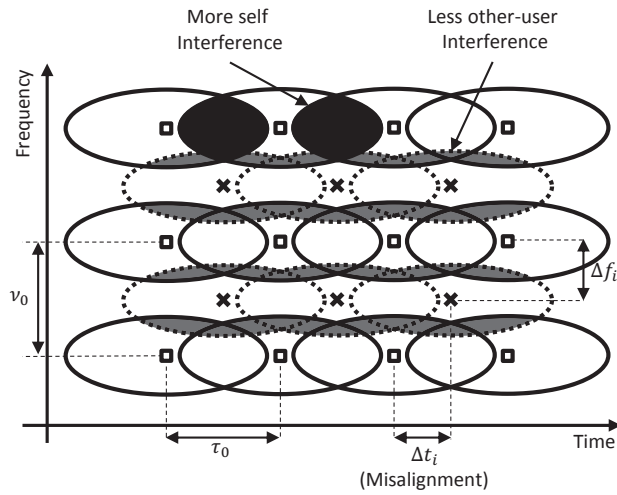
(b) More self-interference, but less other-user-interference.
